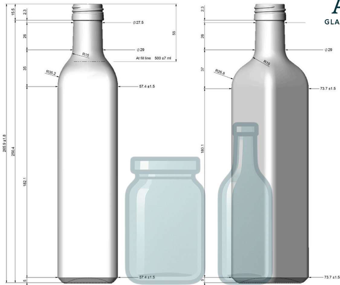
FRONT VIEW
