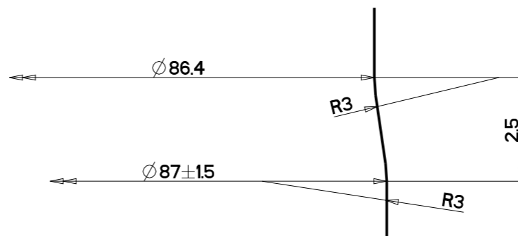
DETALLE A / DETAIL A ESCALA / SCALE : 8/1
